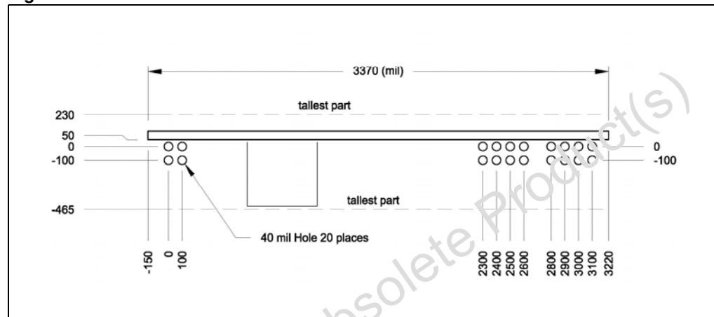
Figure 3. Footprint
