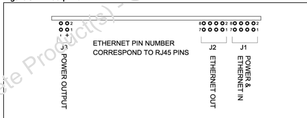
Figure 3. Footprint
